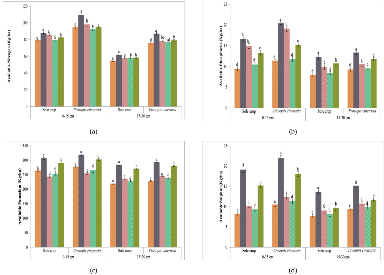
Fig 2. Depth wise values of various soil parameters (a) N, (b) P, (c) K and (d) S for sole crop and P. cineraria based agroforestry systems [values with different letters within a group differed significantly ( p < 0.05 ) from each other]
